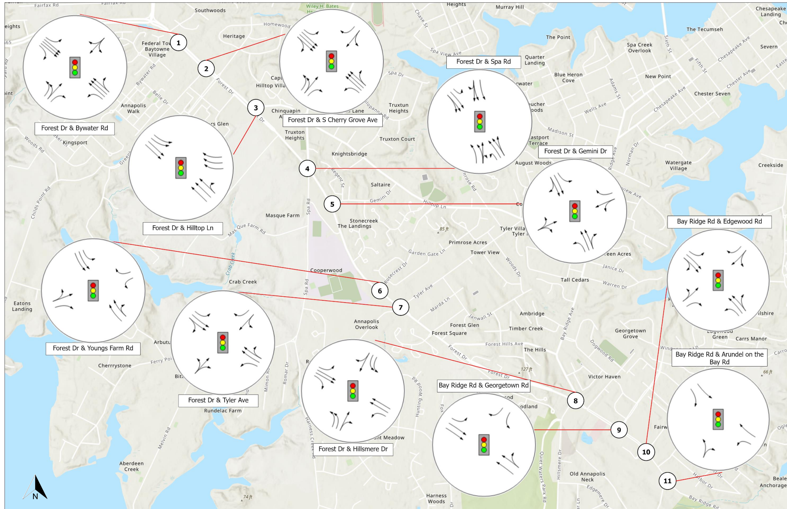
FIGURE 4-1: LANE CONFIGURATION AT SIGNALIZED INTERSECTIONS
