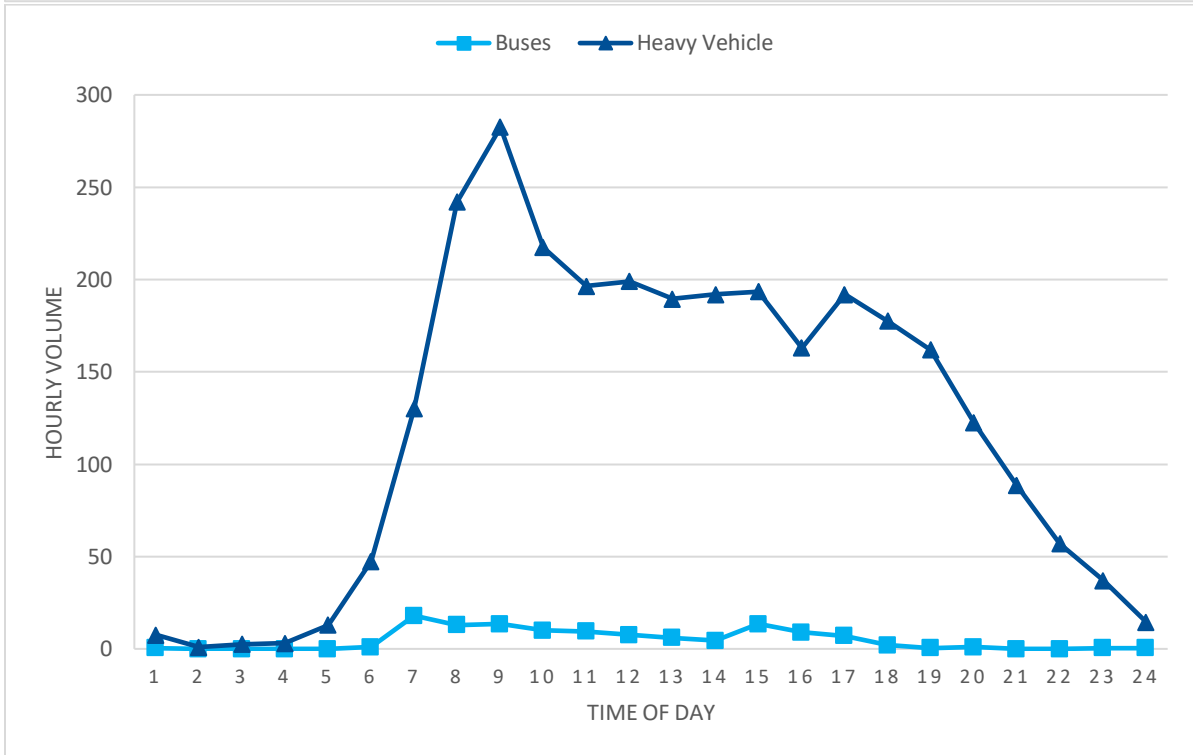
FIGURE 3-7: VEHICLE CLASSIFICATION EAST OF HILLTOP LANE
