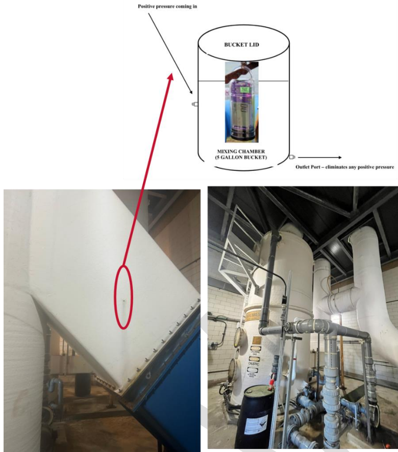
Figure 2-4 Existing non-operational scrubber and the proposed location to install H 2 S monitor.
