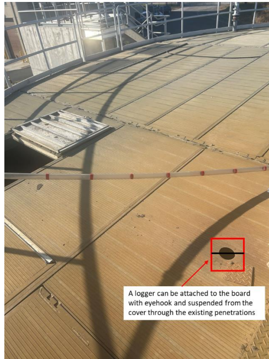
Figure 2-6 Gravity sludge thickener PPM monitor location
