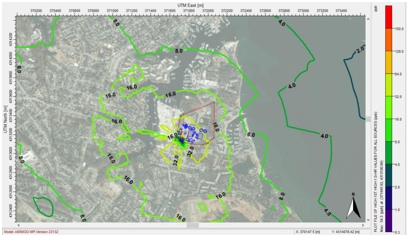
Figure 3-10: All Sources – Scenario 2 Maximum Modeled H 2 S Impacts (ppb).
