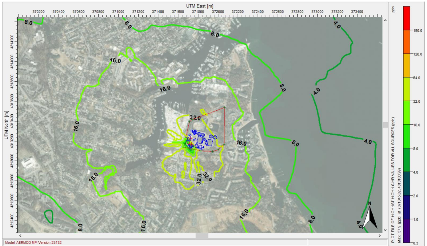
Figure 3-12: All Sources – Scenario 4 Maximum Modeled H 2 S Impacts (ppb)
